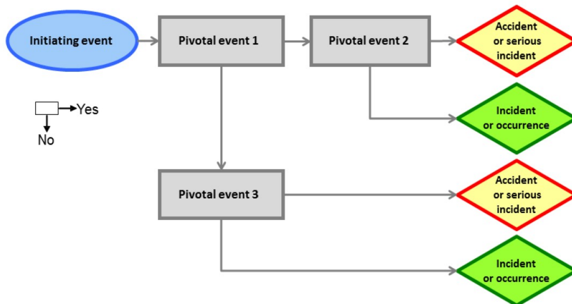
Figure 1: Generic representation of an Event Sequence Diagram.
